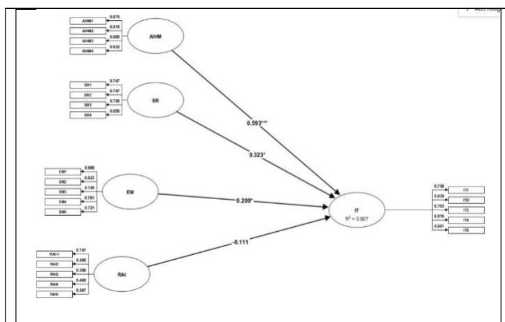
Figure:7 The structural equation modelling of AI in International finance
